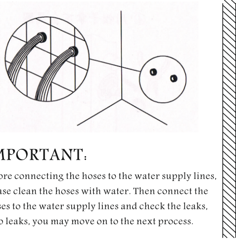
The following picture is the installation constructions of the handheld shower wand.
